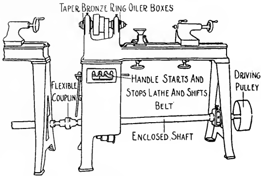
FIG. 201. UNDER DRIVEN LATHE.
